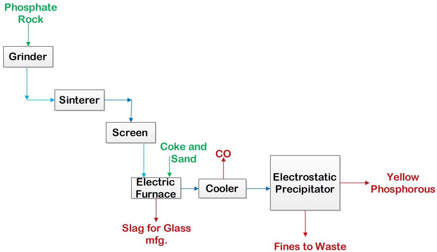
Figure: Manufacturing of Yellow Phosphorous
